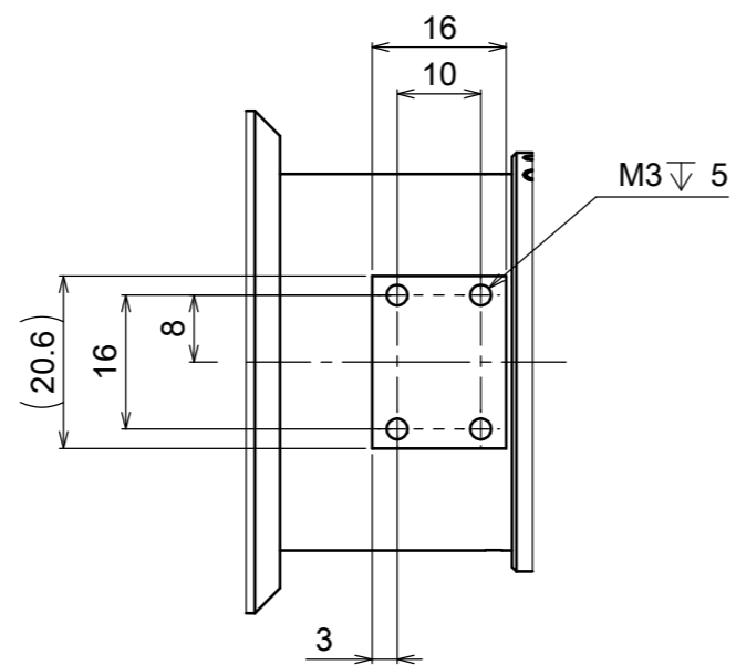
VIEW A (1:1)
