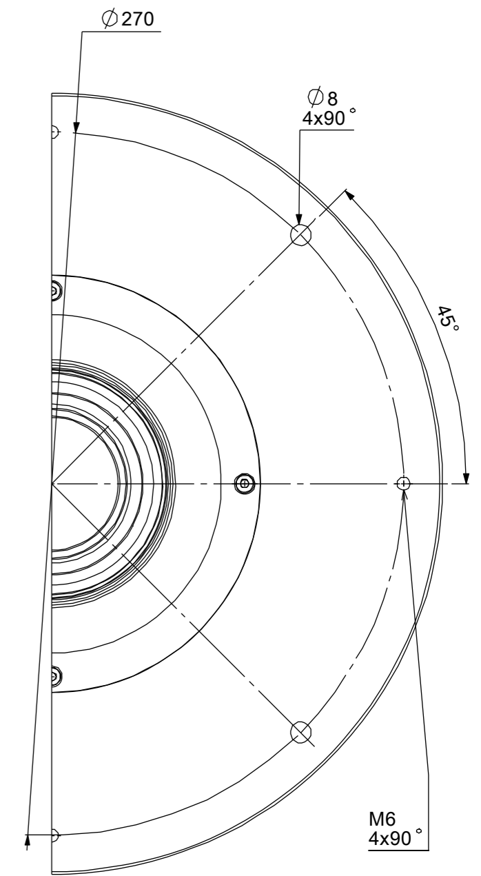
MOUNTING PORTION DETAIL VIEW フランジ取付部詳細
