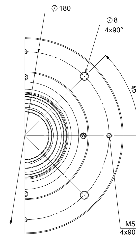
MOUNTING PORTION DETAIL VIEW フランジ取付部詳細
