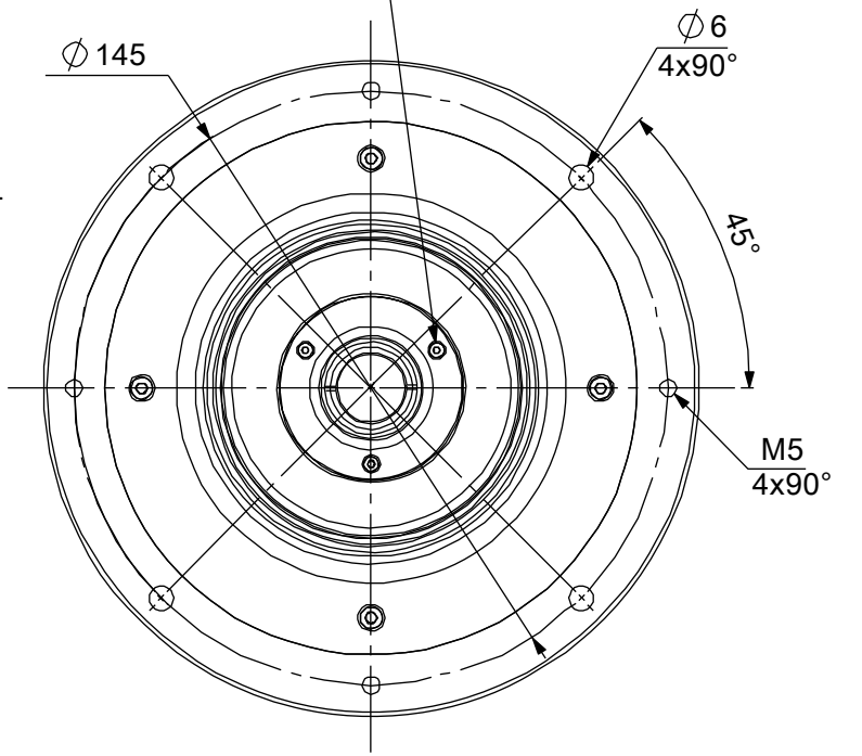
MOUNTING PORTION DETAIL VIEW フランジ取付部詳細
